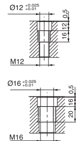
Steel bush Reference No. 2575
