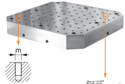
Threaded body Reference No. 2510
