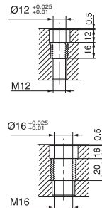
Steel bush Reference No. 2520
