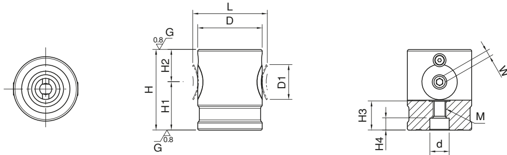
Product Nr. 0950 5-Axis Clamping Block Extension
