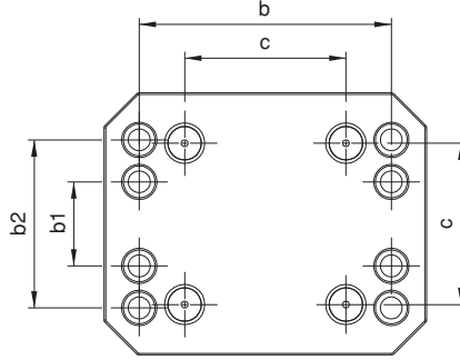
Product Nr. 2316 ER-EL Point Clamp
