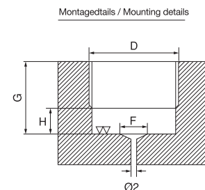
Spanndiagramm Mounting Diagram
